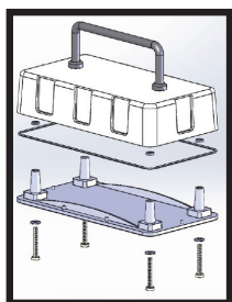
PORTABLE - with Handle
